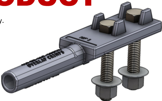
Captive Hardware / Hot-Stick Option
