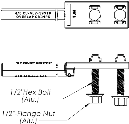
Captive Hardware / Hot-Stick Option
